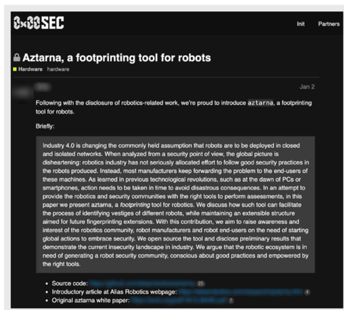
Figure 19. A post about a free tool for discovering industrial robots
